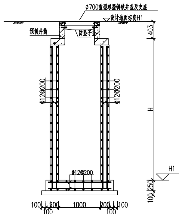
1-1 1:50 (钢筋图)
